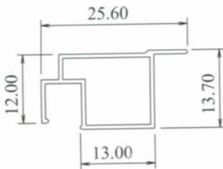
IS154/SJ154 0.165 kg/m AP: 92.18 mm
